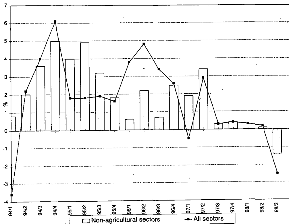
Figure 1: Growth in real gross domestic product at factor incomes: seasonally adjusted annual rates
