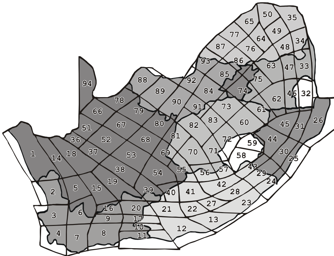
Rainfall districts
